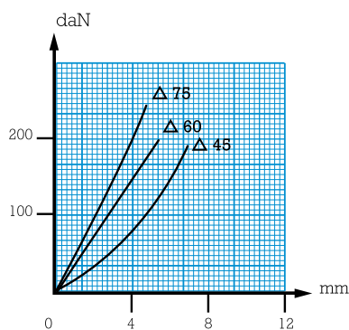
BECA φ 100
