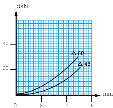
BECA φ 40
