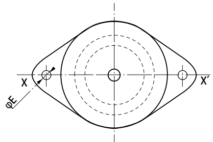
Fig b BECA 底角带安装孔,平孔
